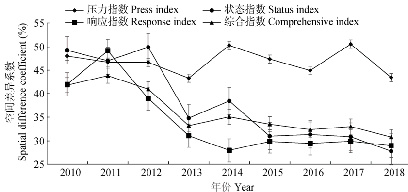
图 3 河北省土地生态安全指数空间差异性 Fig. 3 Space difference of land ecological security index in Hebei Province
