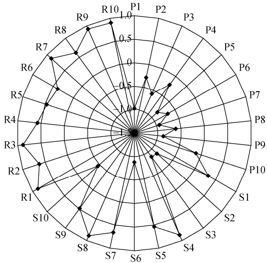
图 2 河北省土地生态安全综合指数与各评价指标相关性 Fig. 2 Correlation between land ecological security index and each evaluation index in Hebei Province 各评价指标名称见表 1。The names of the indexes are shown in the table 1.
